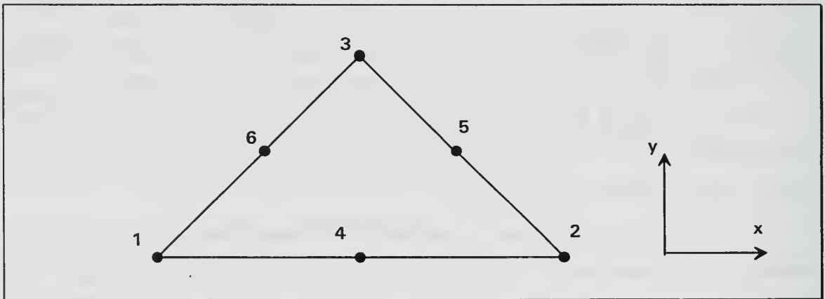
Figure 4. TRIA06R Element Topology. After Ref.[3]
